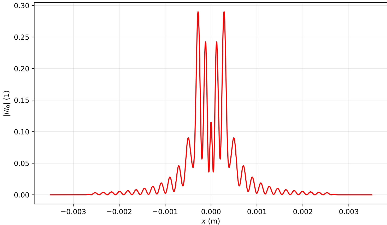
Intensity profile I(x, y = 0, z = 0.159)/I_0 , \text{Pin}=7.0\text{Pcr} , artificial time
